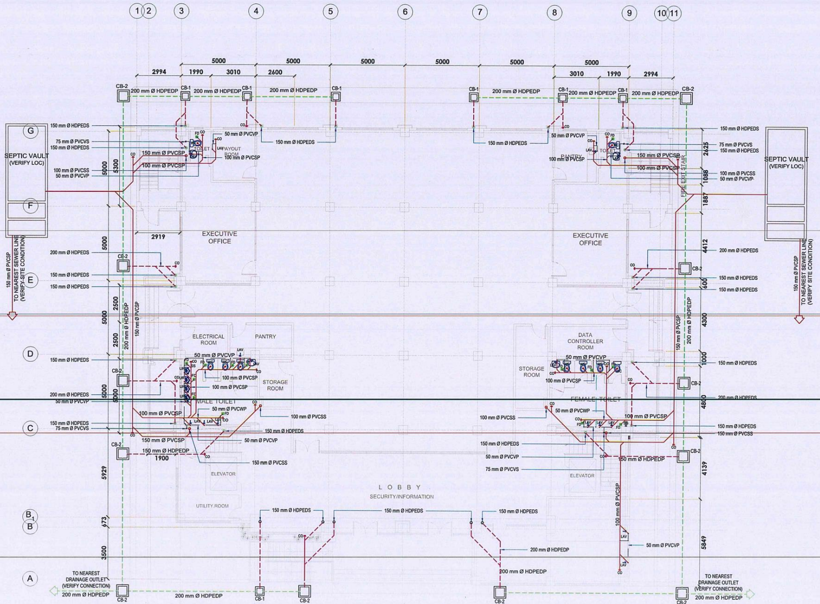
1 GROUND FLOOR PLAN (SEWER AND DRAINAGE LAYOUT) P-1 SCALE 1:100 m.
