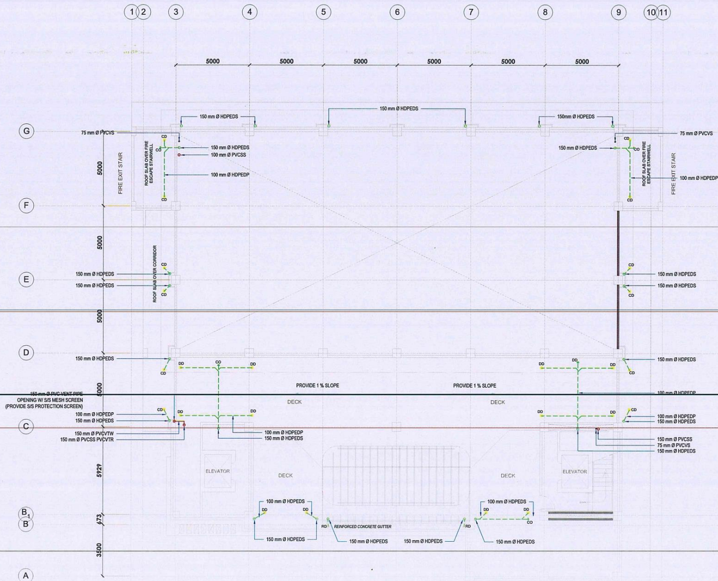
1 P-5 DECK ROOF PLAN (SEWER AND DRAINAGE LAYOUT) SCALE 1 : 100 m.
