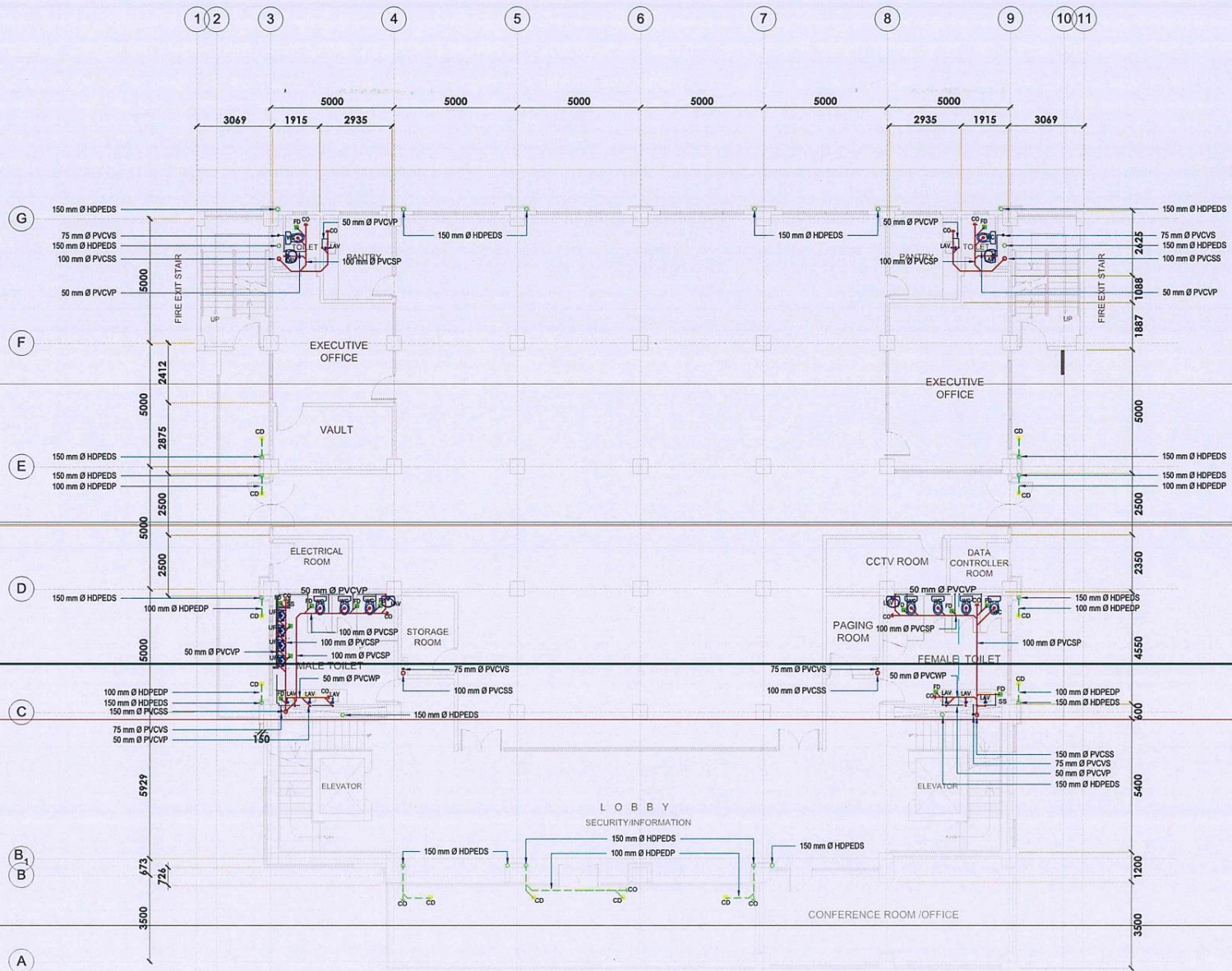
1 SECOND FLOOR PLAN (SEWER AND DRAINAGE LAYOUT) P-2 SCALE 1:100 m.
