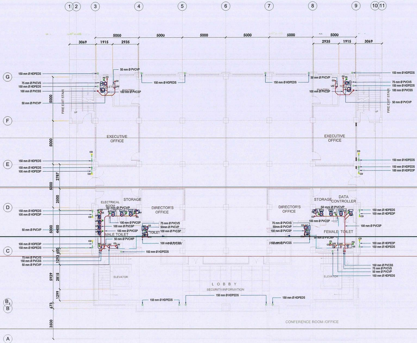
1 THIRD FLOOR PLAN (SEWER AND DRAINAGE LAYOUT) P-3 SCALE 1:100 m.
