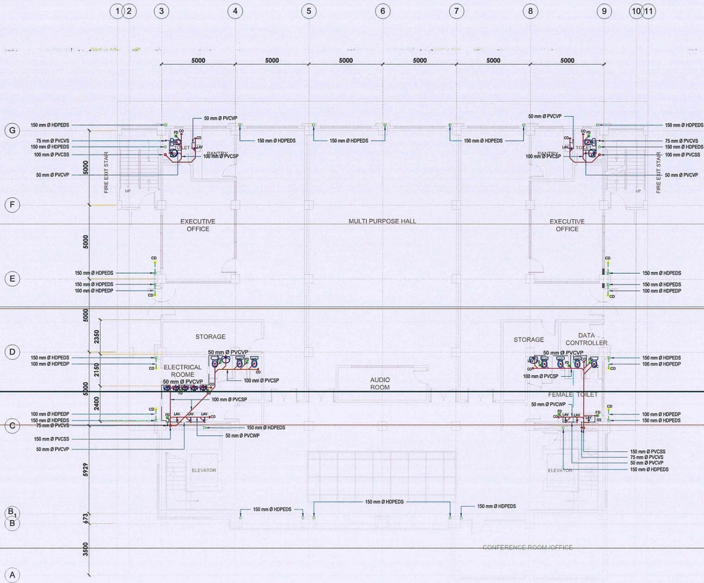
1 FOURTH FLOOR PLAN (SEWER AND DRAINAGE LAYOUT) P-4 SCALE 1:100 m.
