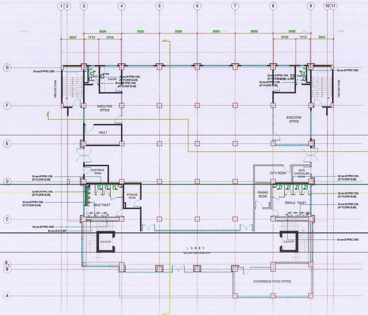
SECOND FLOOR COLD WATER SUPPLY SYSTEM PLAN SCALE 1:100 MTS
